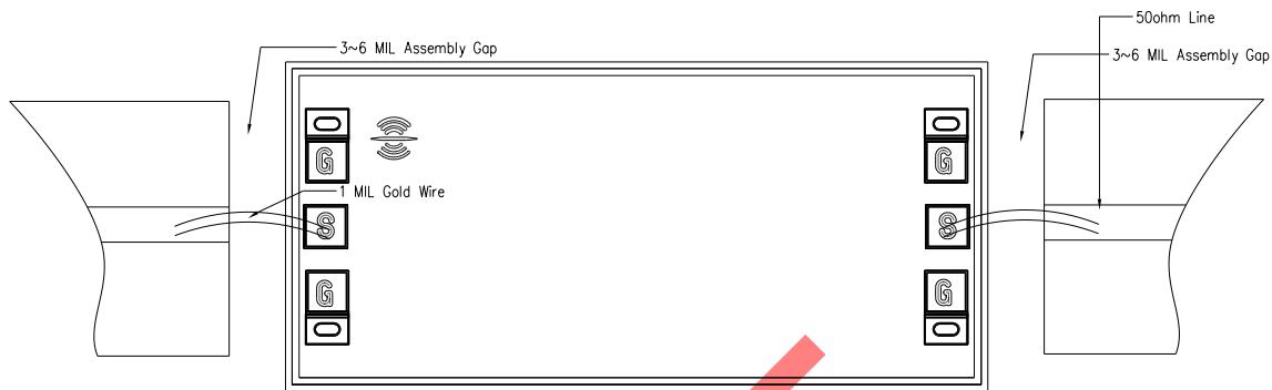
Assembly Diagram
