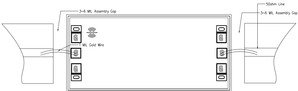
Assembly Diagram
