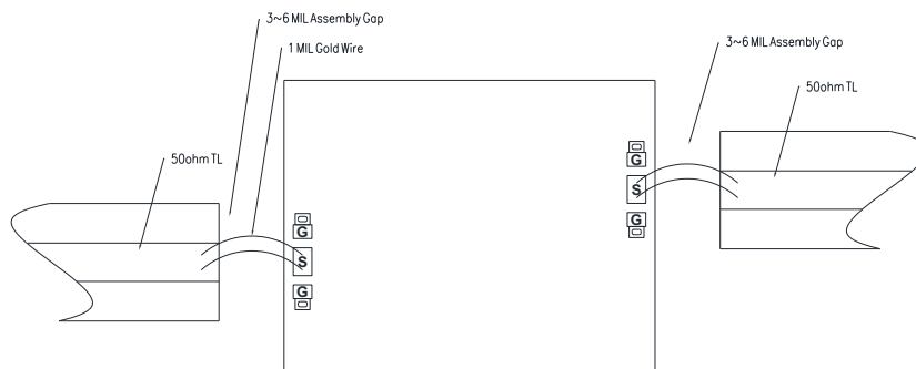
Assembly Diagram
