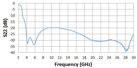
Return Loss vs. Frequency
