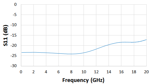
Return Loss vs. Frequency
