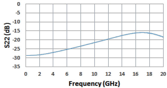
Return Loss vs. Frequency
