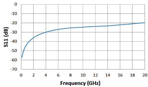
Retrun Loss vs. Frequency
