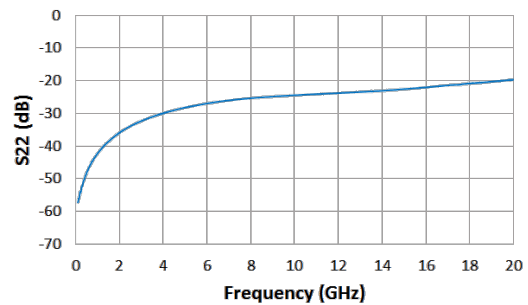
Retrun Loss vs. Frequency
