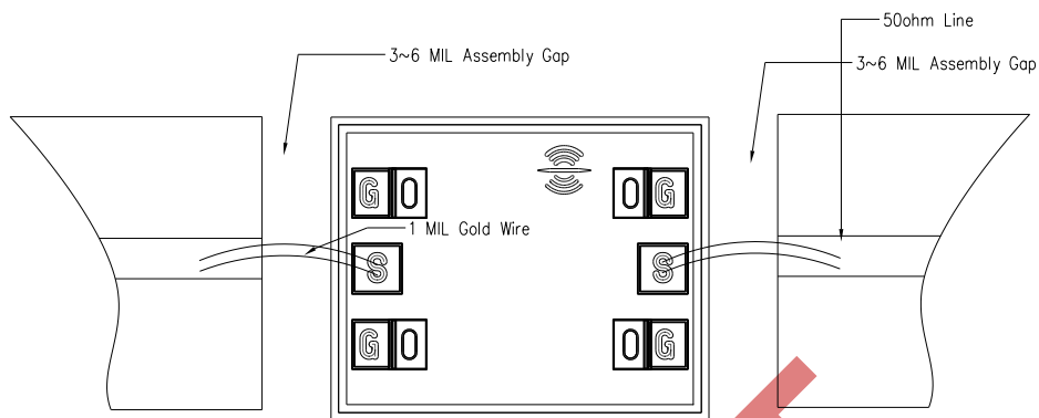
Assembly Diagram
