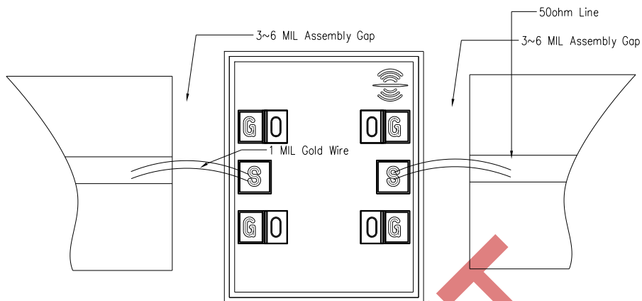
Assembly Diagram
