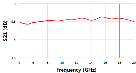
Insertion Loss vs. Frequency
