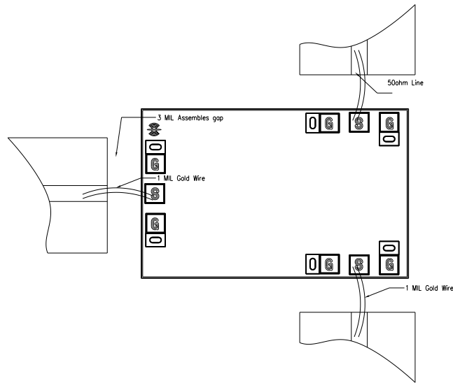
Assembly Diagram
