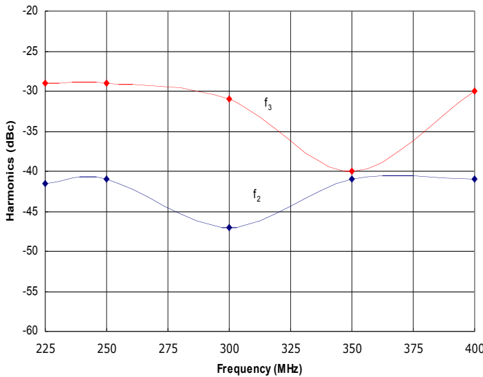
Figure 3: HD31372 Typical f 2 and f 3 @ P out =50W.
