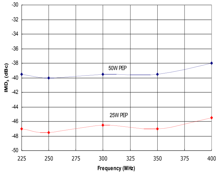
Figure 2: HD31372 Typical IMD 3 @ 50W and 25W PEP, Δf=10kHz and Δf=100kHz.
