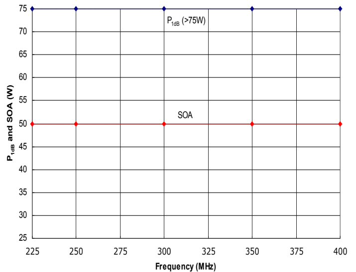
Figure 4: HD31372 Typical P 1dB and Safe Operating Area (SOA). The amplifier is capable of delivering much more power than it is safe to generate. Do not exceed the SOA shown above without first contacting HD Communications Corp. to discuss your application.
