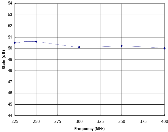
Figure 1: HD31372 Typical Gain @ P out =50W.
