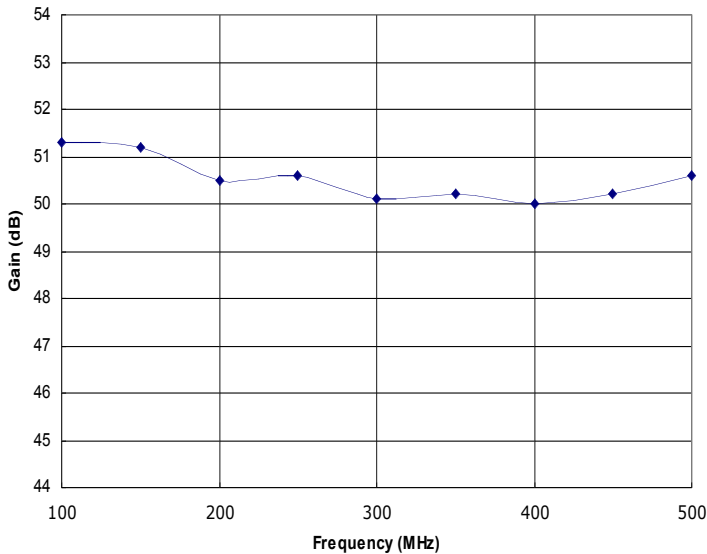
Figure 1: HD31349 Typical Gain @ P_{out}=50W .
