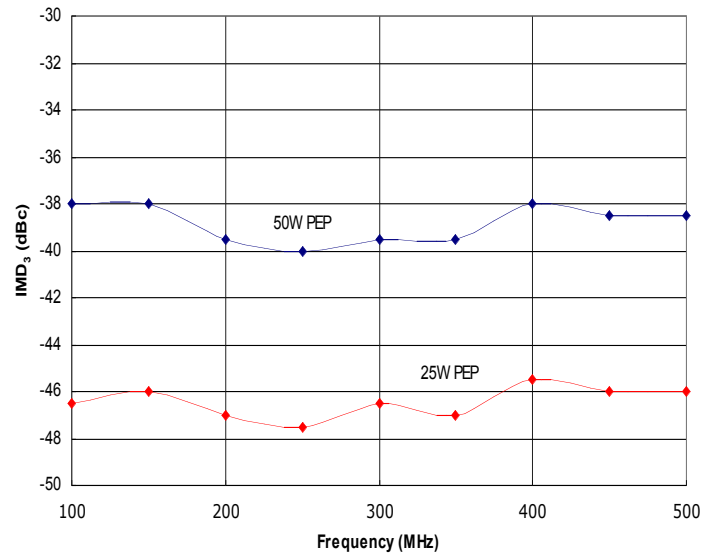
Figure 2: HD31349 Typical IMD 3 @ 50W and 25W PEP, \Delta f=10kHz and \Delta f=100kHz .
