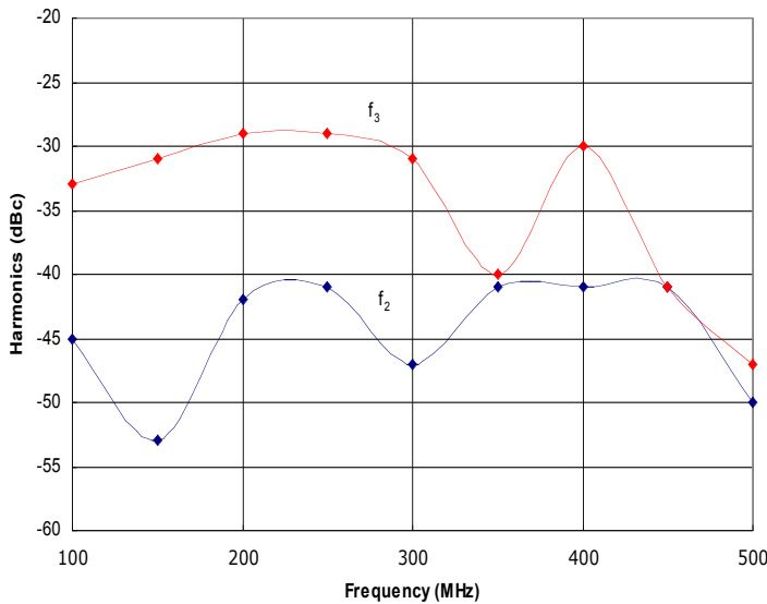
Figure 3: HD31349 Typical f_2 and f_3 @ P_{out}=50W .
