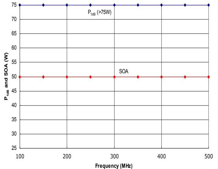
Figure 4: HD31349 Typical P_{1dB} and Safe Operating Area (SOA). The amplifier is capable of delivering much more power than it is safe to generate. Do not exceed the SOA shown above without first contacting HD Communications Corp. to discuss your application.
