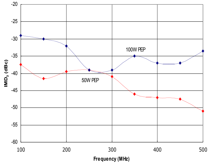
Figure 2: HD31348 Typical IMD 3 @ 100W and 50W PEP, Δf=10kHz.
