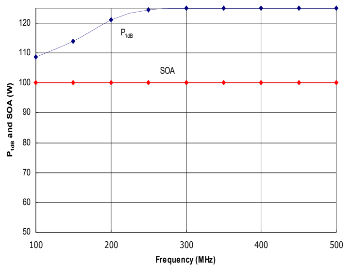
Figure 4: HD31348 Typical P 1dB and Safe Operating Area (SOA). Do not exceed the SOA shown above without first contacting HD to discuss your application.
