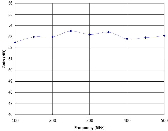
Figure 1: HD31348 Typical Gain @ P out =100W.
