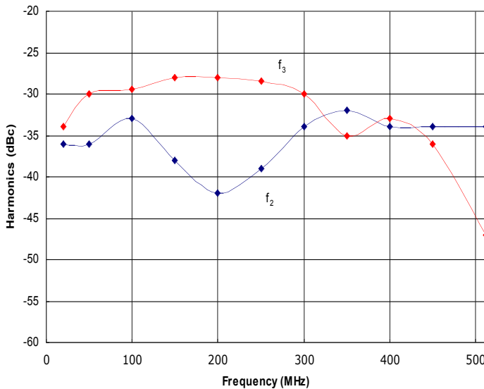
Figure 3: HD31342 Typical f_2 and f_3 @ P_{out}=50W .
