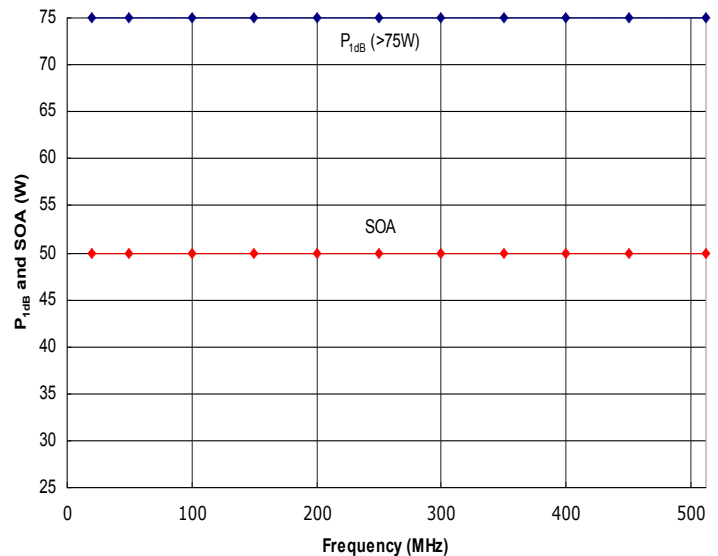
Figure 4: HD31342 Typical P_{1dB} and Safe Operating Area (SOA). The amplifier is capable of delivering much more power than it is safe to generate. Do not exceed the SOA shown above without first contacting HD Communications Corp. to discuss your application.
