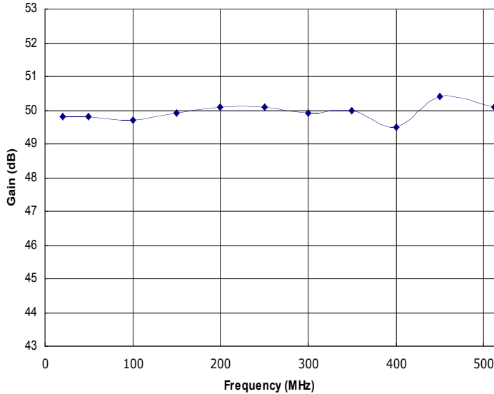
Figure 1: HD31342 Typical Gain @ P_{out}=50W .
