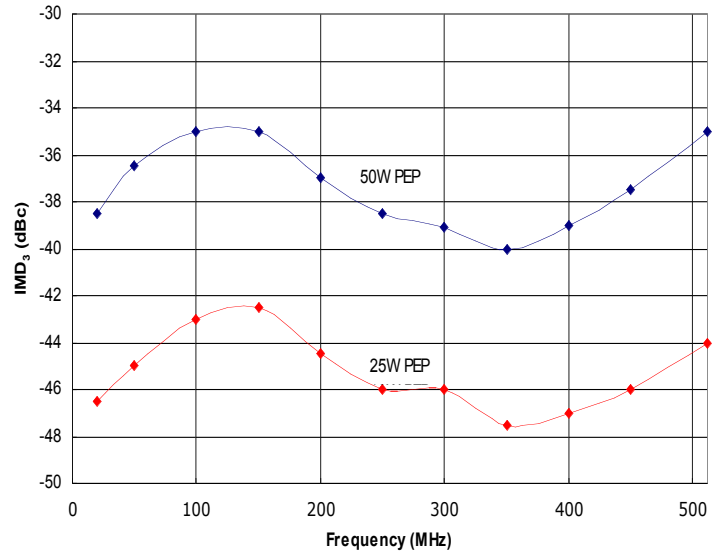
Figure 2: HD31342 Typical IMD_3 @ 50W and 25W PEP, \Delta f=10kHz and \Delta f=100kHz .
